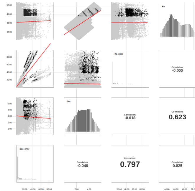
Figure 9: Brushing
