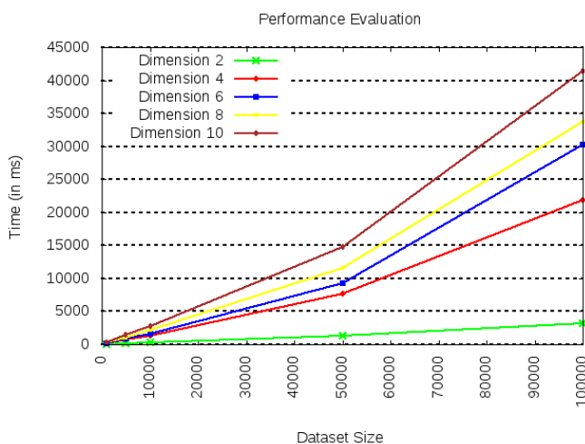
Figure 10: Performance Evaluation
