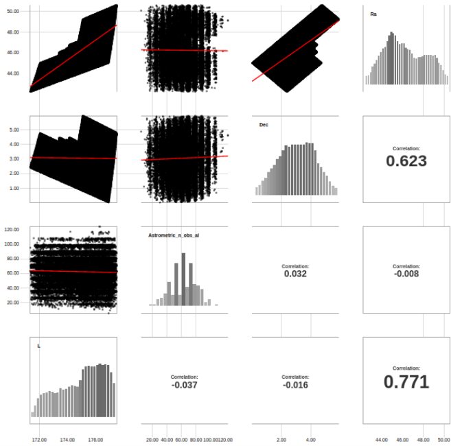
Figure 7: Scatterplotmatrix
